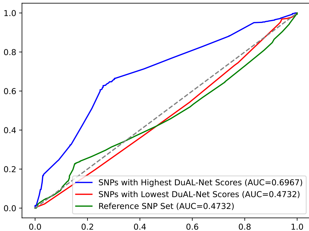
ROC for n=100
