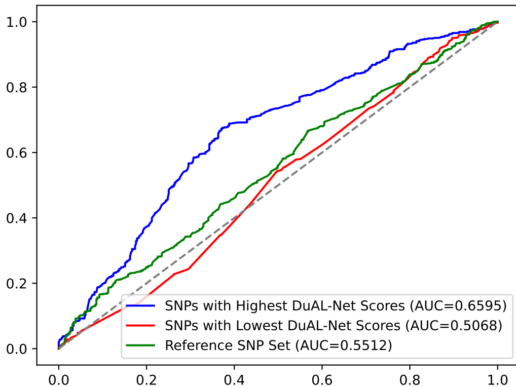
ROC for n=500
