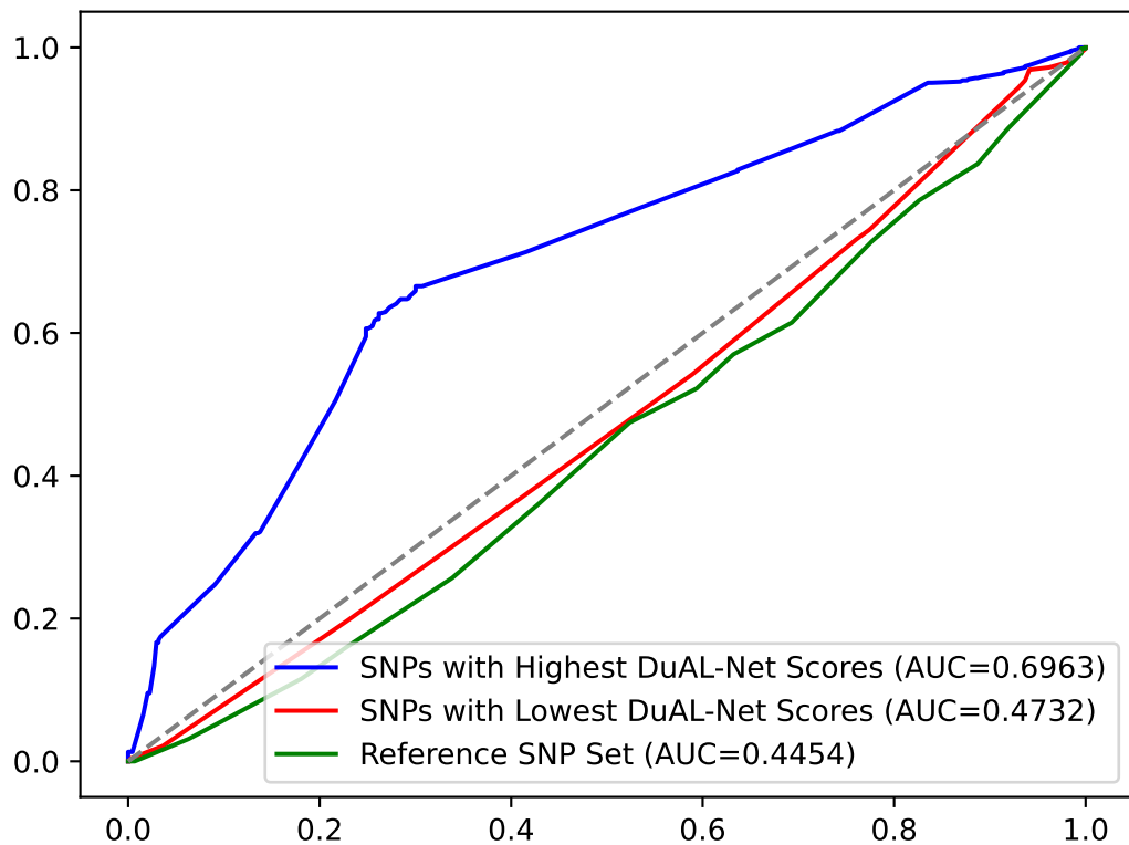
ROC for n=50
