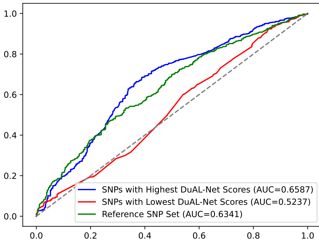
ROC for n=1000
